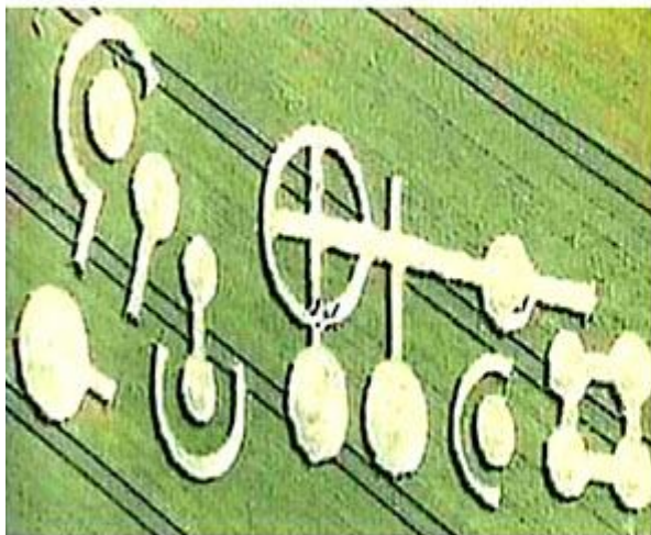
Grasdorf, Germany 1991
