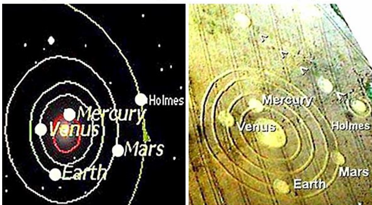
May 4, 2007 (perihelion)
