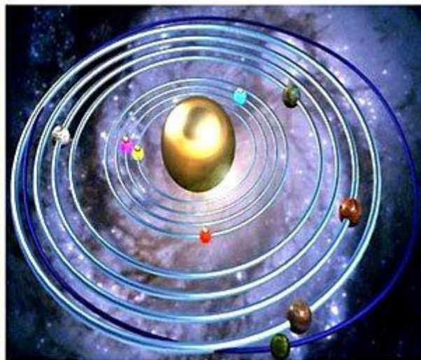
our solar system on December 23, 2012
