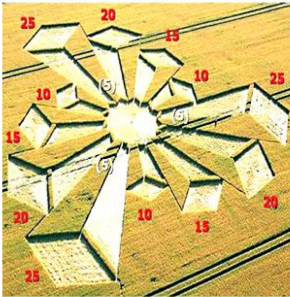
Wayland's Smithy 2006
