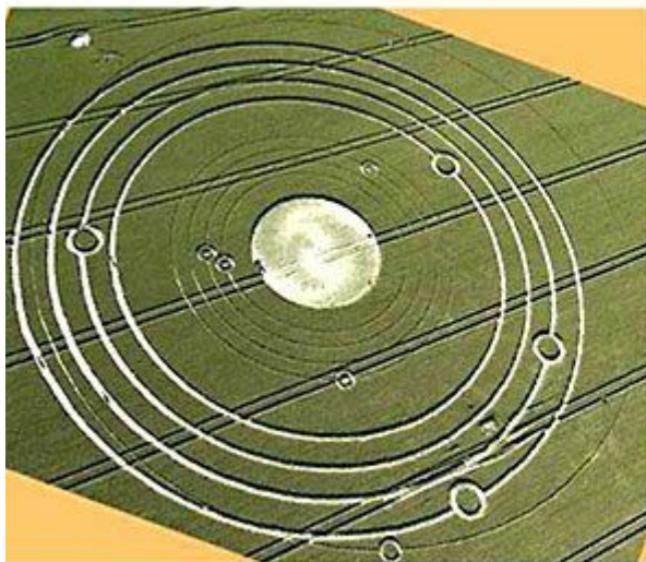
Avebury Manor 2008
