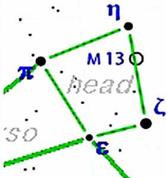
Hercules and M13
