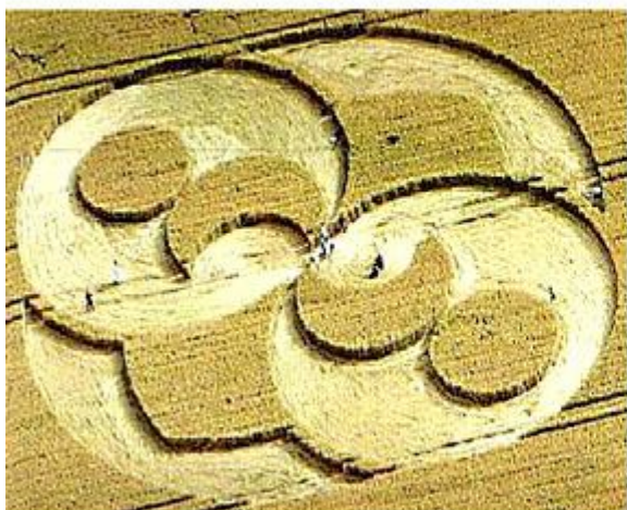
Chiseldon 1996
